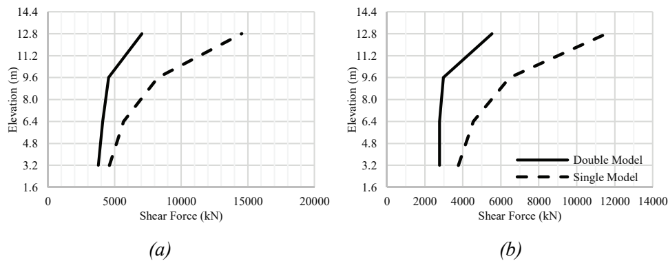
Figure 11 - Diaphragm shear force distribution per unit length of slab at +12.80 m elevation of double model obtained from RSA.
