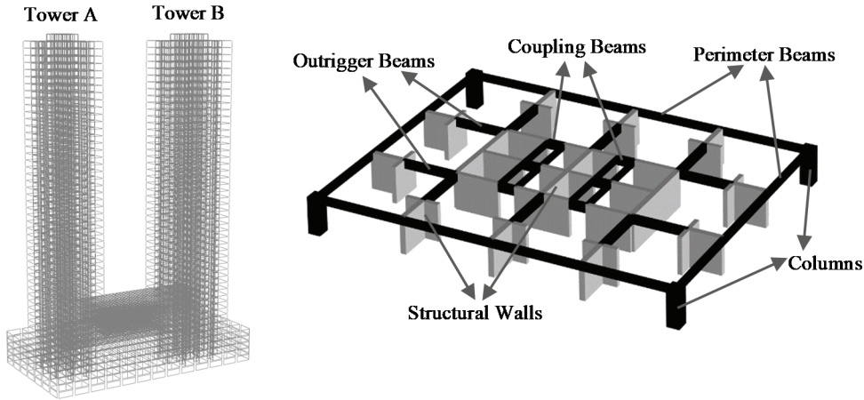
Figure 4 – Nonlinear double-tower model geometry and nonlinear structural elements.
