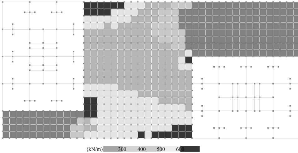
Figure 19 - Diaphragm tensile force distribution (in X direction) per unit length of slab at +12.80 m elevation of double model obtained from NLRHA under record RSN1762 [14].
