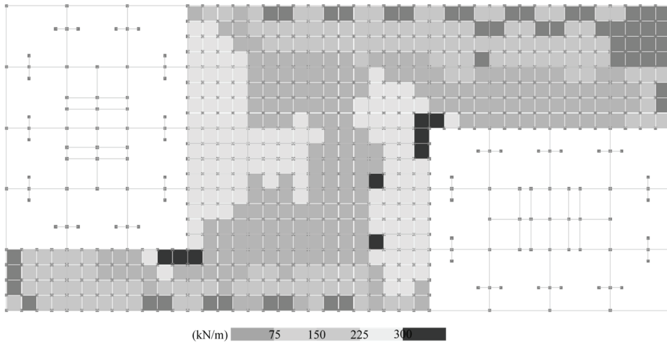
Figure 21 - Diaphragm shear force distribution per unit length of slab at +12.80 m elevation of double model obtained from NLRHA under RSN1762 [14] record.
