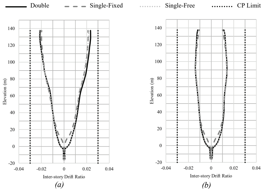
Figure 24 - Comparison of NLRHA interstory drift ratio distributions for double, single-fixed and single-free models of Tower A at (a) DA-X, (b) DA-Y.
