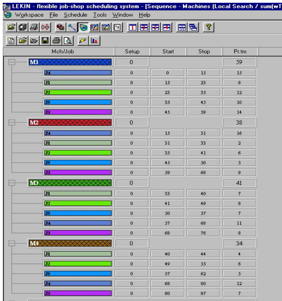
Figure 6: Sequence Scheme of the Local Search Algorithm
