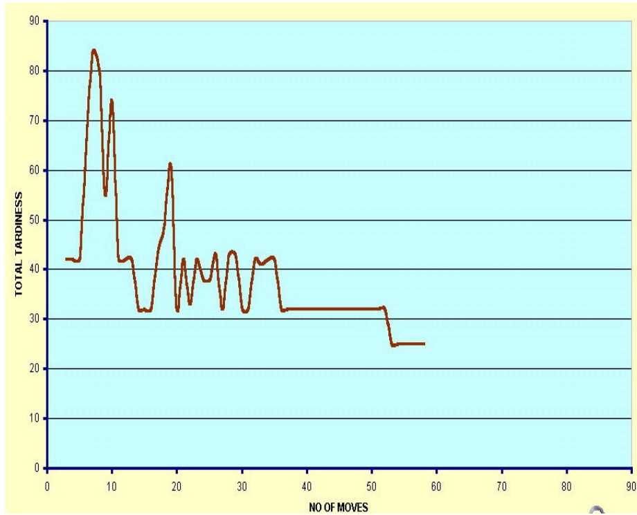
Figure 3: Changes On Total Weighted Tardiness During The Neighborhood Search
