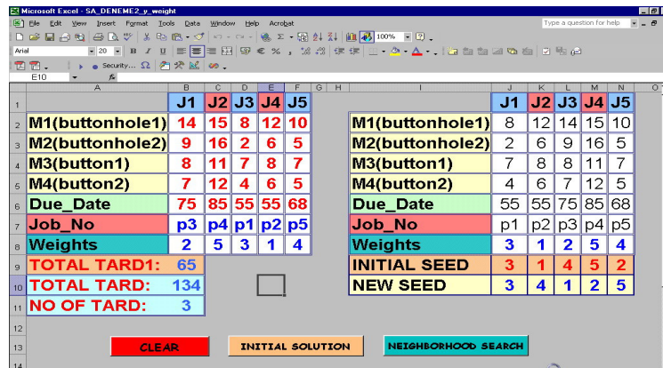
Figure 2: User-interface of Excel Application Sheet
