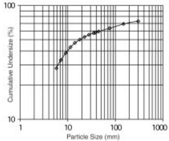
Figure 2: Particle size distribution of İvrindi alunitic kaolin
