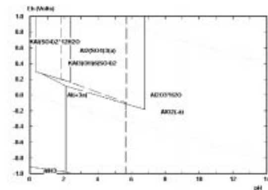
Figure 5: Eh-pH diagram of Al-K-S-H 2 O system at 25 °C (dashed lines show the aqueous phase)
