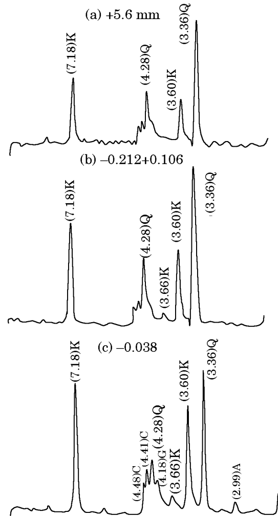
Figure 4: XRD patterns of some particle size fractions of İvrindi alunitic kaolin
