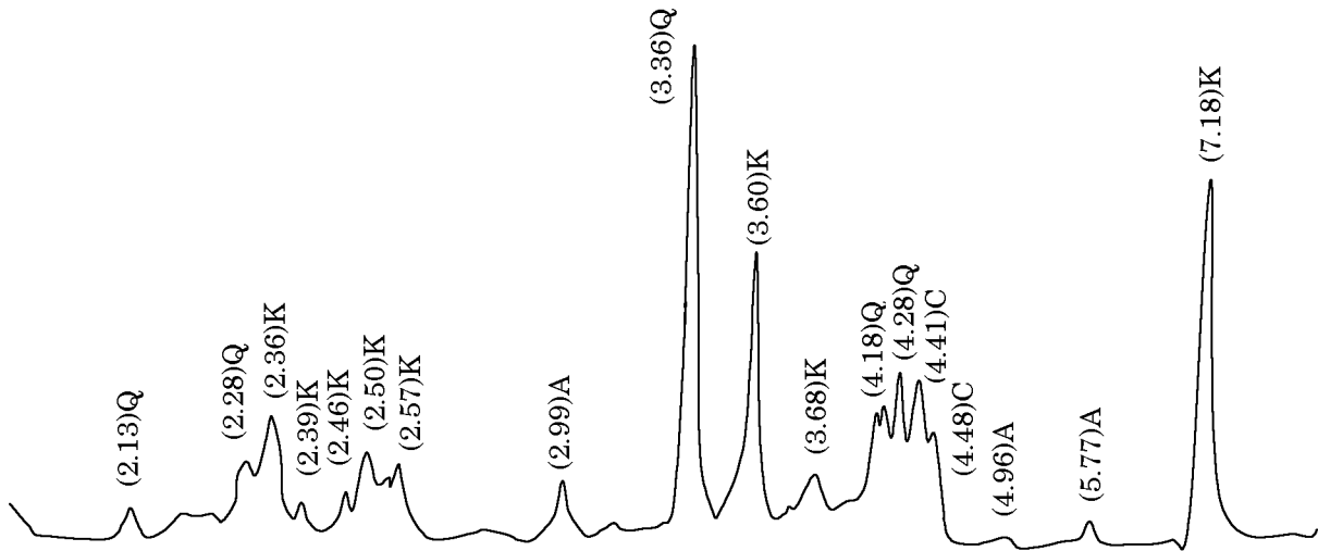
Figure 1: XRD pattern of İvrindi alunitic kaolin
