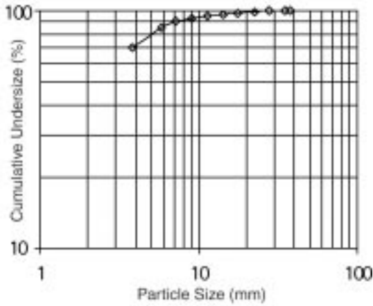
Figure 3: Particle size distribution of the cyclone overflow product
