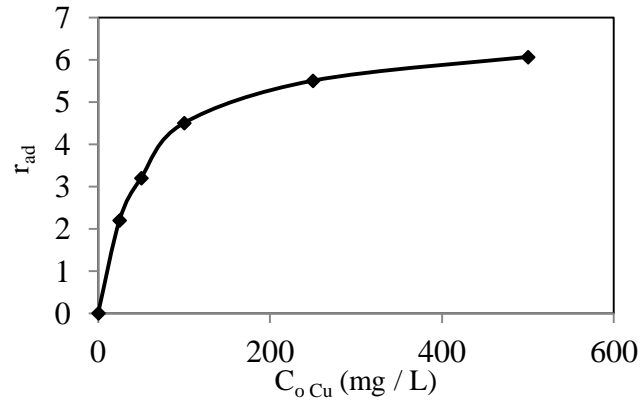
Figure 3. Effect of initial Cu (II) ion concentration on adsorption rate at pH 5.0 for bentonite
