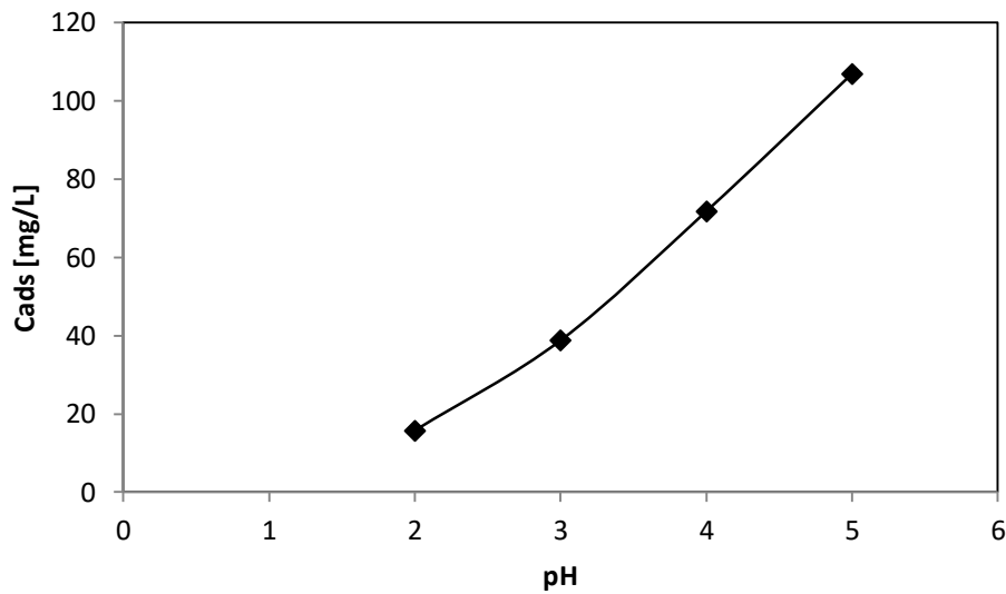
Figure 2. Adsorption-induced effect of initial pH on the adsorption of Cu (II) ions for Bentonite (T: 23 ° C)
