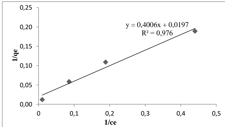
Figure 5. Adsorption isotherm obtained by linearization of the Langmuir adsorption isotherm equation at pH 5.0 for bentonite and Cu (II) (T: 23 ° C)
