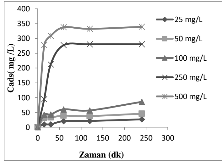
Figure 4. Adsorption-time graph of Cu (II) ions with bentonite
