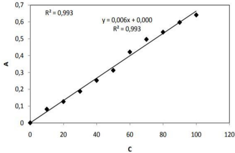
Figure 1. The working line used for Cu (II) ion concentration determination
