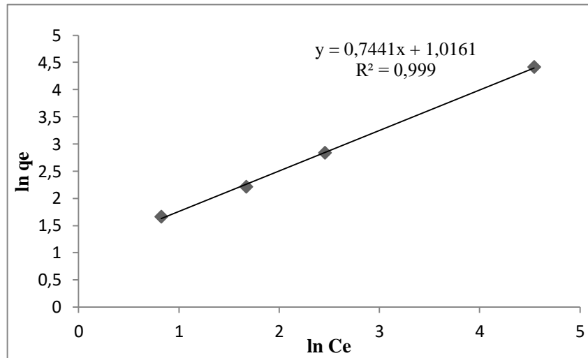
Figure 6. Adsorption isotherm obtained by linearization of Freundlich adsorption isotherm equation at pH 5.0 for bentonite and Cu (II) (T: 23 ° C).
