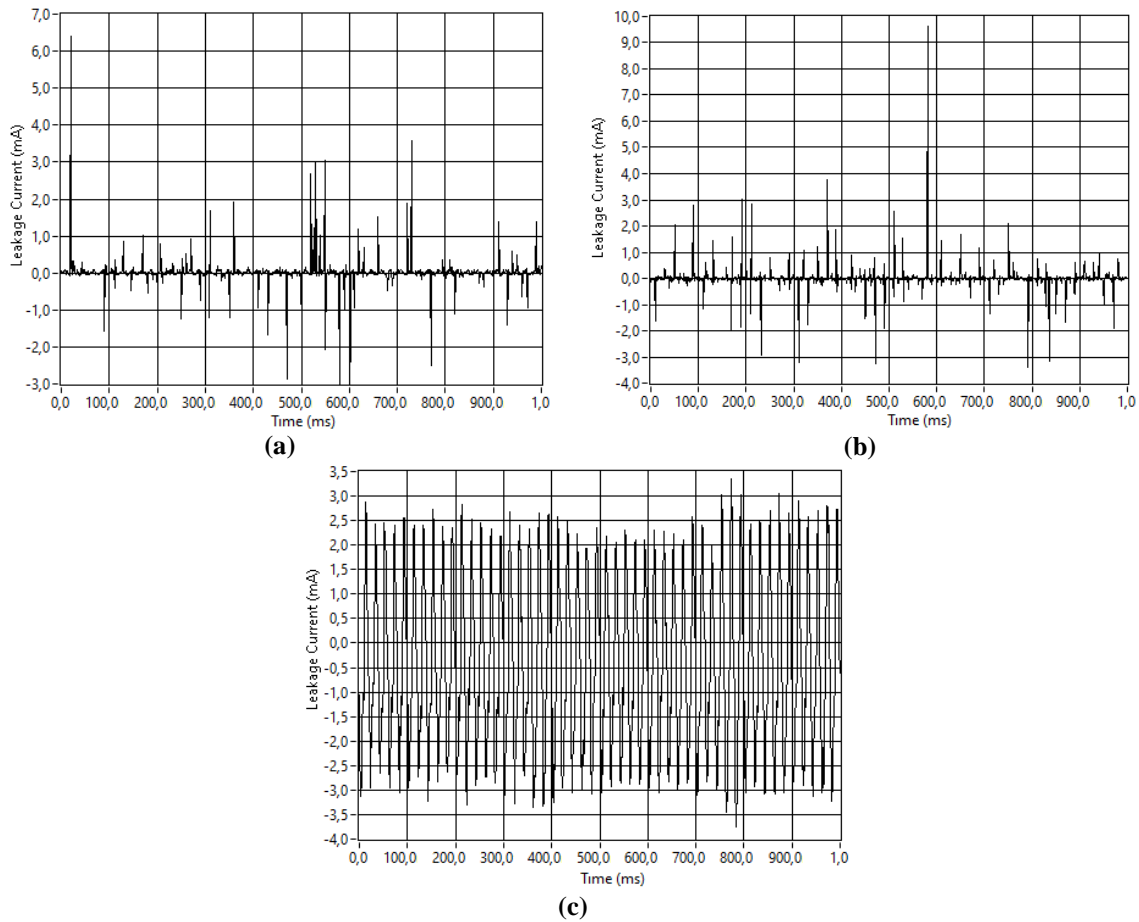
Figure 7. For an iced (a) porcelain, (b) glass, (c) silicone insulator with a conductivity of 4000 \mu\text{S/cm} , the leakage currents obtained under a voltage of 20 kV just before the ice liquefies.
