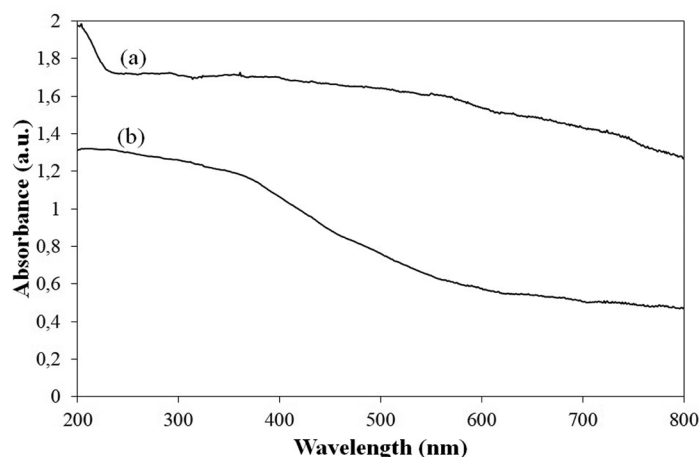
Figure 4. UV-Vis spectra of (a) B_2O_3 and (b) Fe-B_2O_3 .
