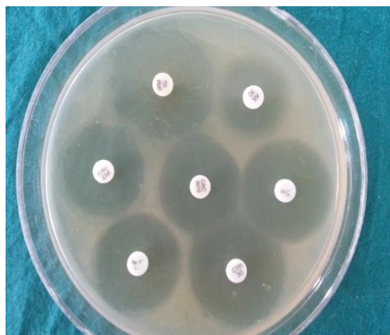
Figure 2: Antibiotic sensitivity test by Kirby Bauer disc diffusion test on 100mm plate.
