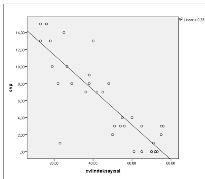
Figure 4. Chart of Correlation between CVP and VCI-CI
