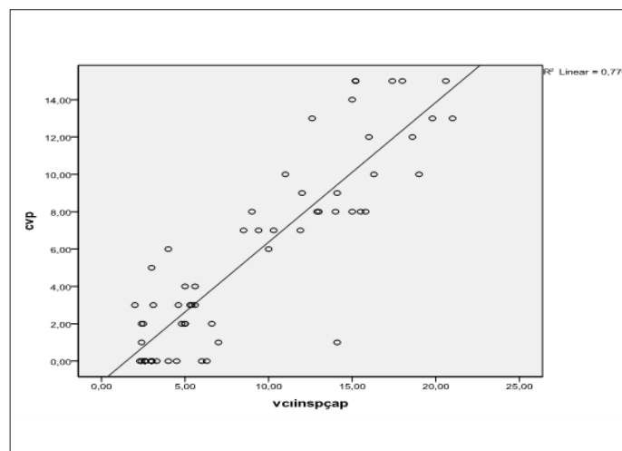
Figure 3. Chart of Correlation between CVP and VCI-i diameter
