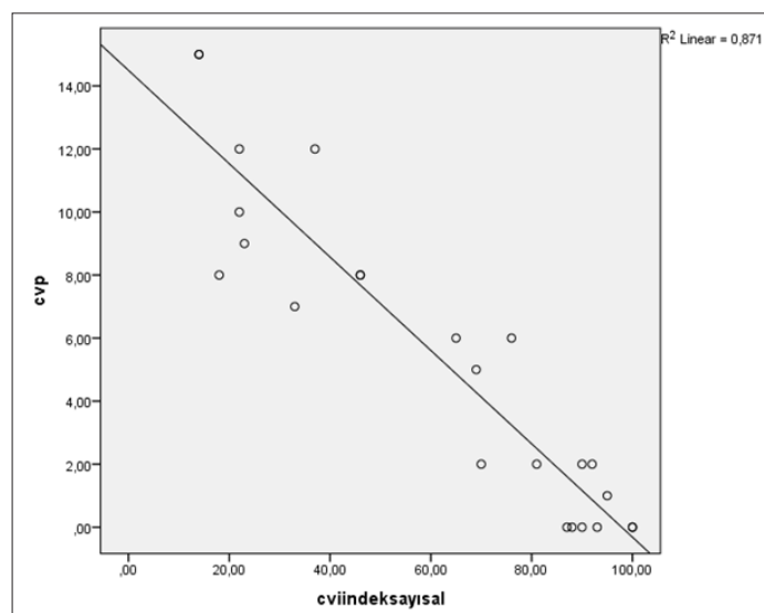
Figure 5. Chart of Correlation between CVP and VCI-DI
