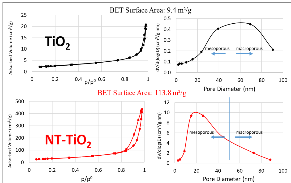
Figure 2. Adsorption-desorption isotherms, pore volume distribution and total surface area values of commercial and prepared NanoTube- \text{TiO}_2
