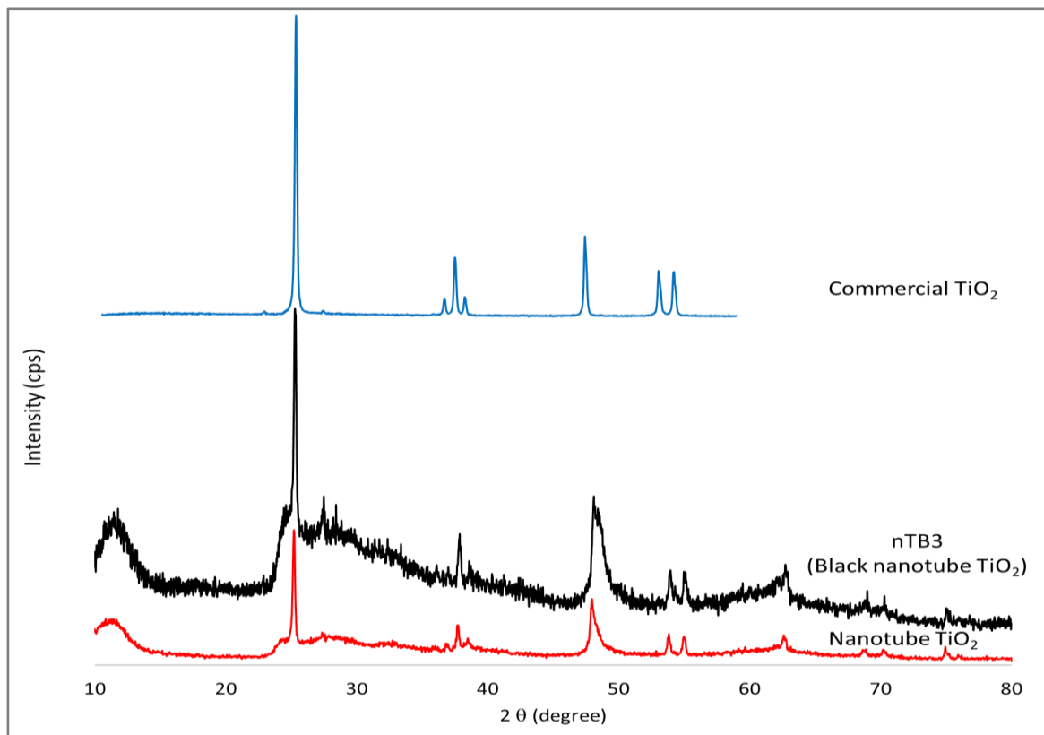
Figure 5. XRD spectra of commercial, nanotube and black nanotube \text{TiO}_2 catalysts
