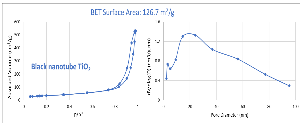
Figure 6. Adsorption-desorption isotherms, pore size distribution and total surface area values of black NanoTube- \text{TiO}_2
