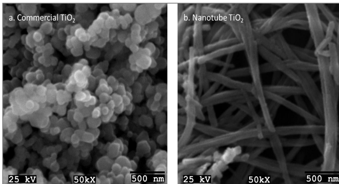
Figure 1. SEM images of a) commercial and b) prepared nanotube \text{TiO}_2
