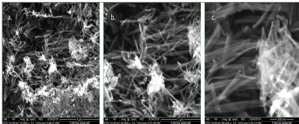
Figure 7. ESEM images of black \text{TiO}_2 a) 4 \mu\text{m} , b) 2 \mu\text{m} and c) 500 nm
