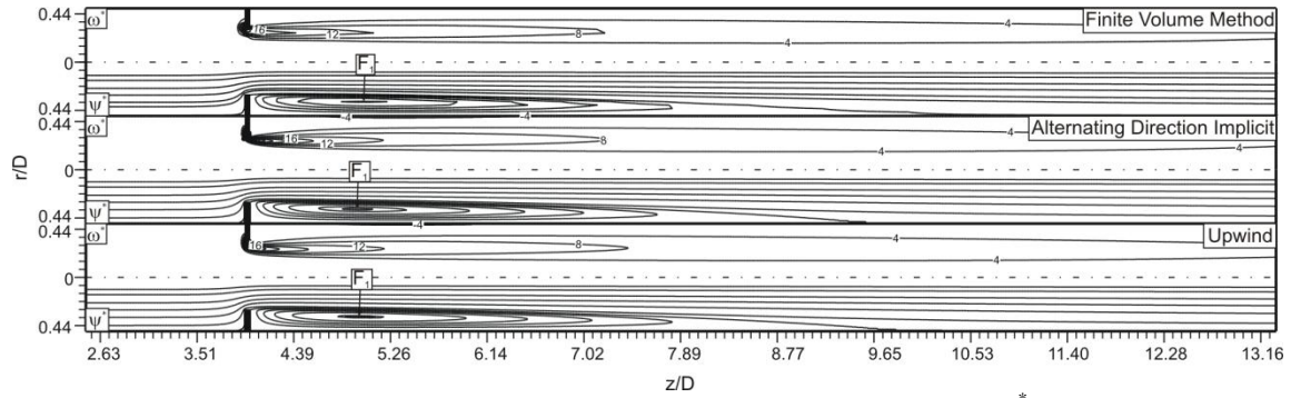
Figure 5. Streamlines and vorticity contours for Re_o=400 , \beta=0.6 and L^*=1/12 .
