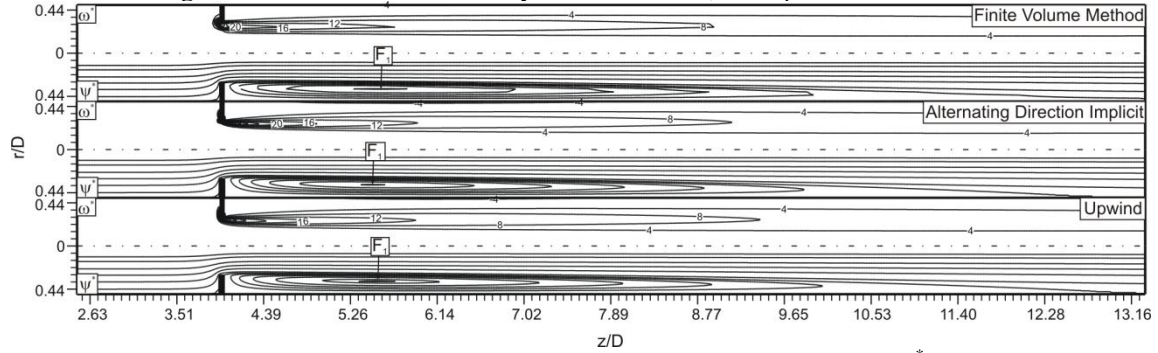
Figure 6. Streamlines and vorticity contours for Re_o=625 , \beta=0.6 and L^*=1/12 .
