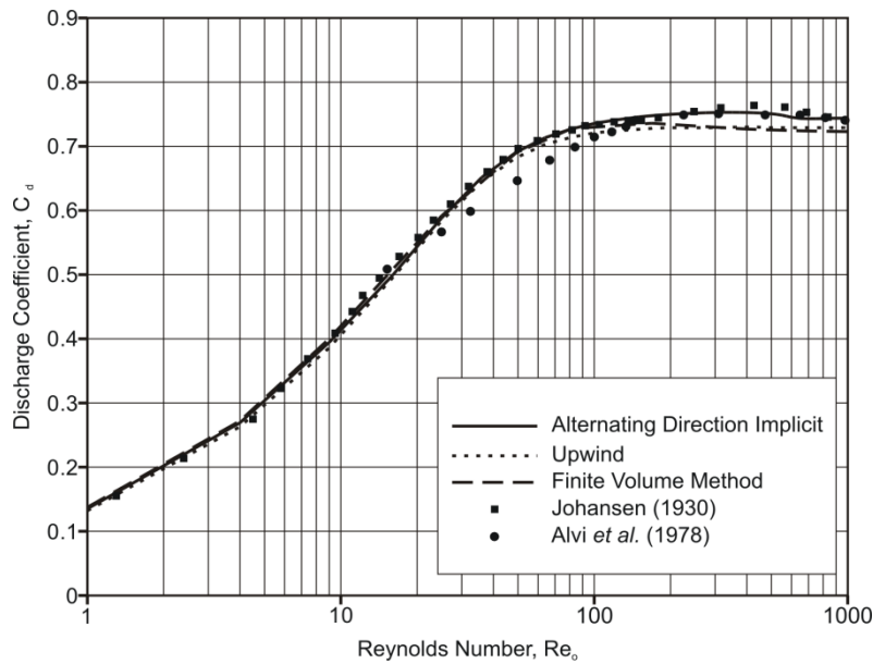
Figure 7. Comparison of the variation of the orifice discharge coefficient with Reynolds number for \beta=0.6 .
