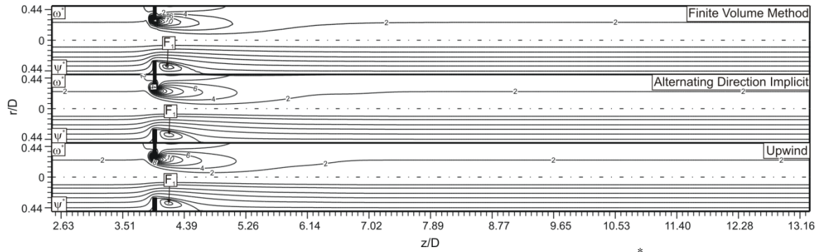
Figure 4. Streamlines and vorticity contours for Re_o=36 , \beta=0.6 and L^*=1/12 .
