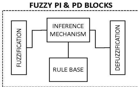
Figure 5.b. The Internal structure of fuzzy PI &amp; PD blocks
