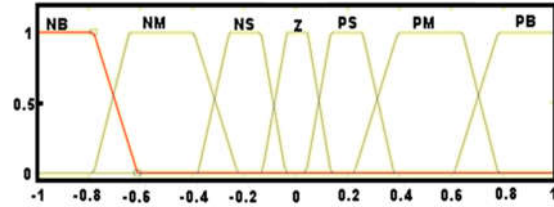
Figure 6. Membership functions for inputs (error, error and error)
