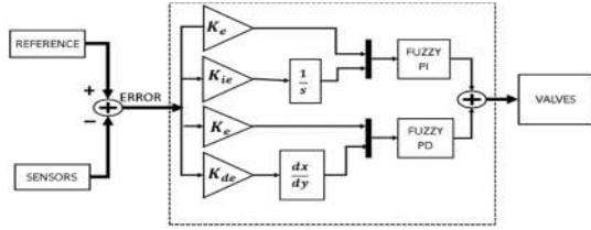
Figure 5.a. Fuzzy PID controller
