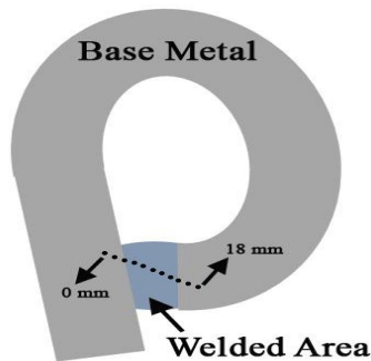
Figure 1. Schematic illustration of rolled and welded steel bar
