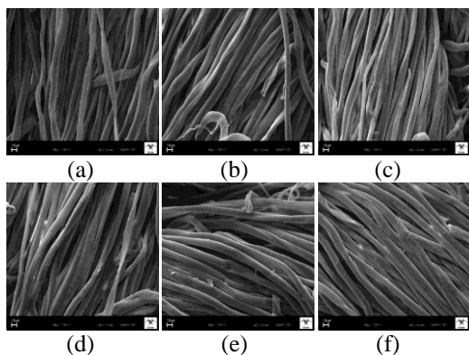
Figure 7. The SEM images of the fabrics (a.1, b.2, c.3, d.4, e.5, f.6) [12]
