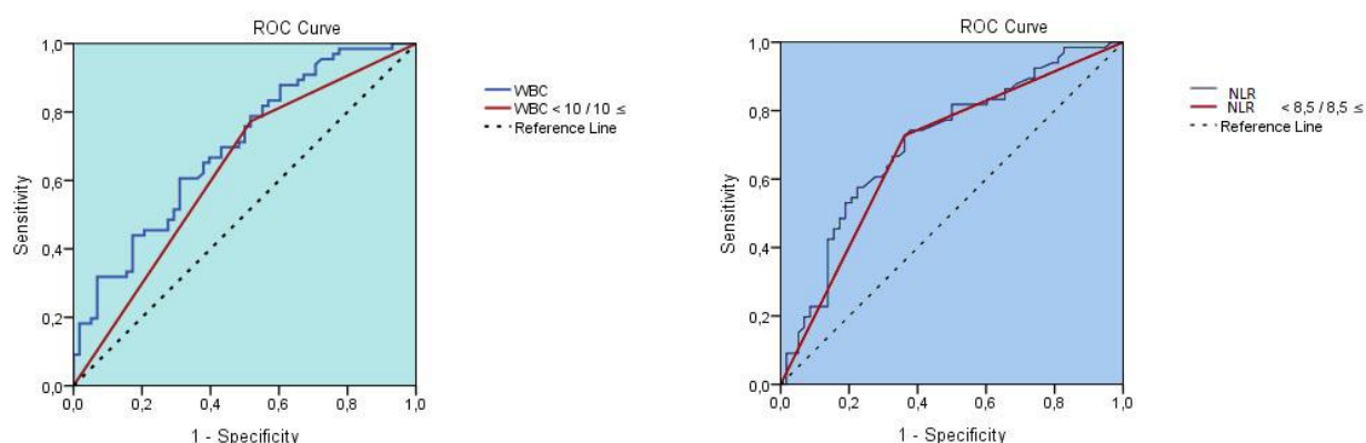
Figure 1. Receiver-operating characteristic (ROC) curve analysis for prediction of postoperative atrial fibrillation (AF) by WBC (white blood cell) and NLR (neutrophil/lymphocyte ratio).
