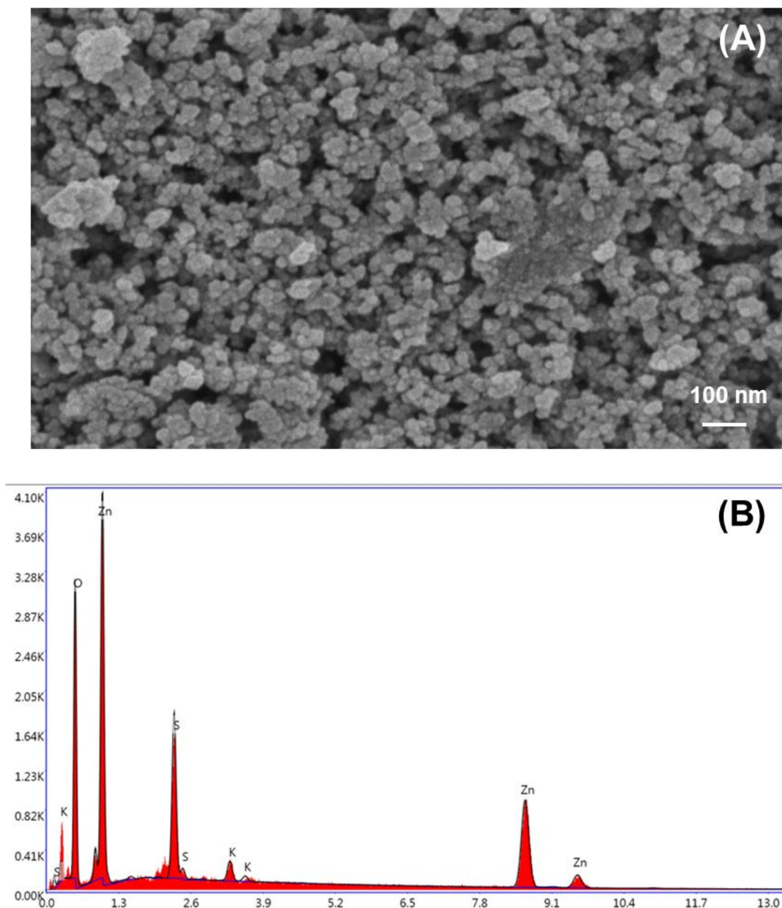
Fig. 6. FE-SEM image and SEM-EDX analysis of ZnO NPs.
