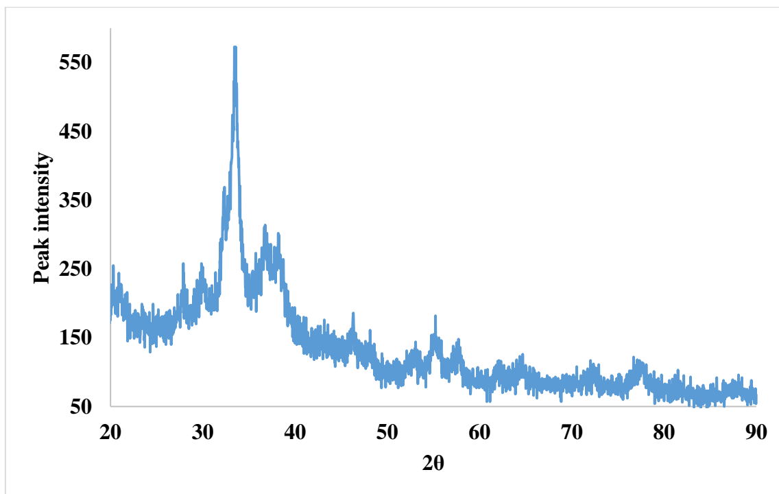
Fig. 1. XRD spectrum of Ag NPs.
