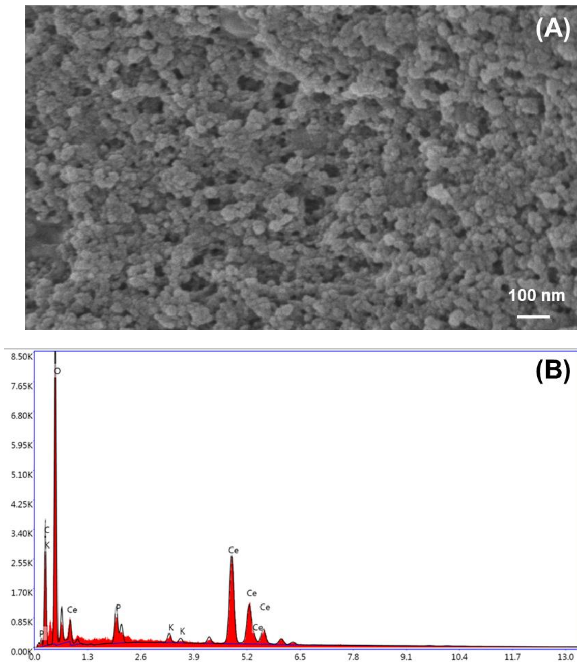
Fig. 4. FE-SEM image and SEM-EDX analysis of \text{Ce}_2\text{O}(\text{CO}_3)_2 \cdot 2\text{H}_2\text{O} NPs.
