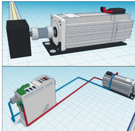
Figure 3. Connections of the motor with the track and the motor drive.
