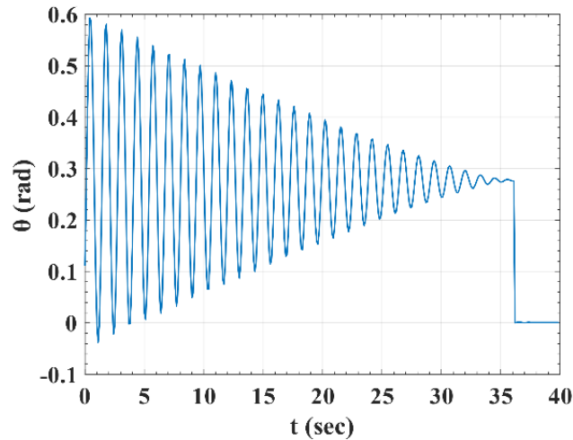
Figure 11. Adjustment of angle reference.
