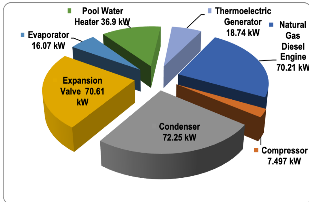
Figure 3. Exergy destructions in the components of the plant
