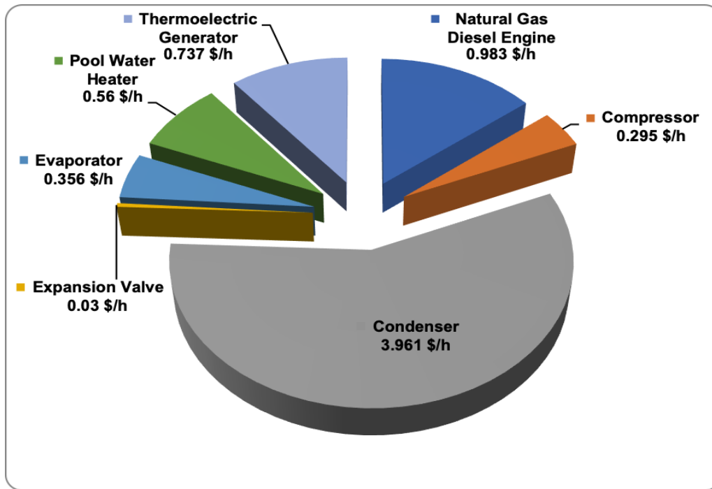
Figure 4. Distribution of exergetic cost destruction rate diagram of the system parts
