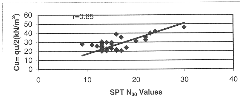
Figure 6. The Correlation of the SPT- N_{30} versus C_u (undrained shear strength) alues
