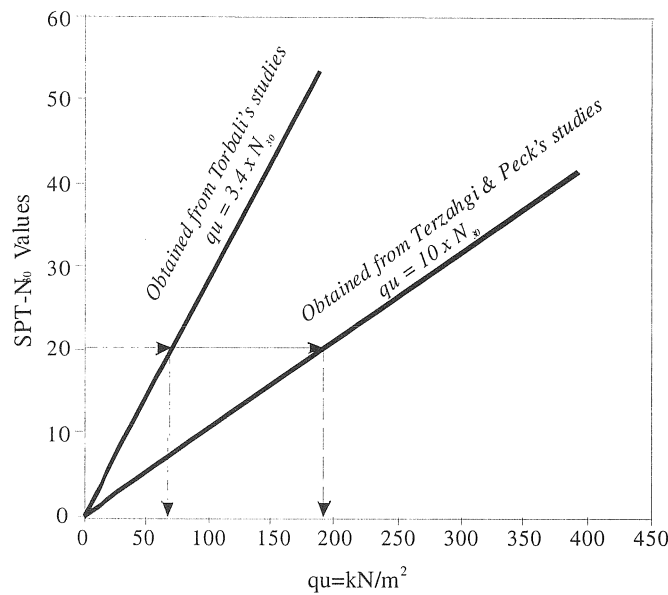
Figure 7 The graphical relationship between SPT- N_{30} , q_u (unconfined ompression strength) and water content values.
