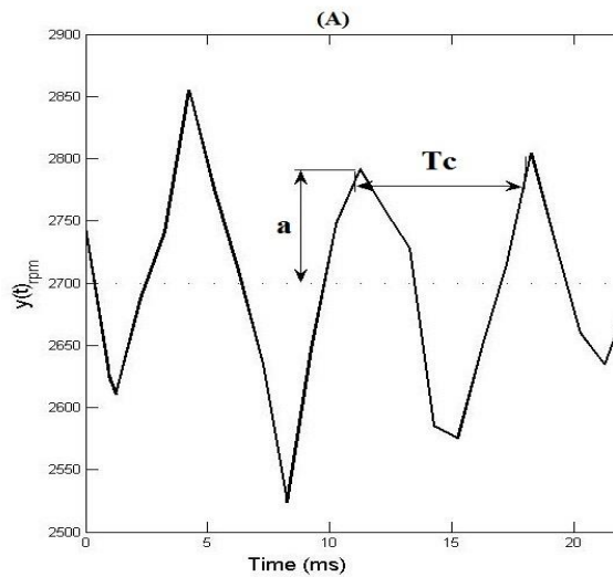
Figure 3. Response signal of the system - y(t) .
