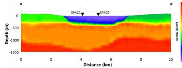
Figure 9. 2D subsurface density model for the A-A' profile.
