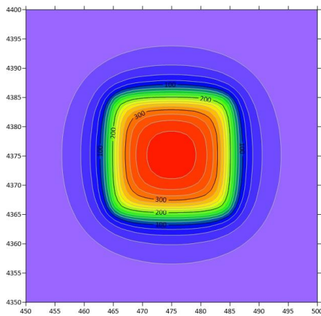
Figure 7. Gravity anomaly map generated using the Potensoft program for the structure in the form of a rectangular prism.
