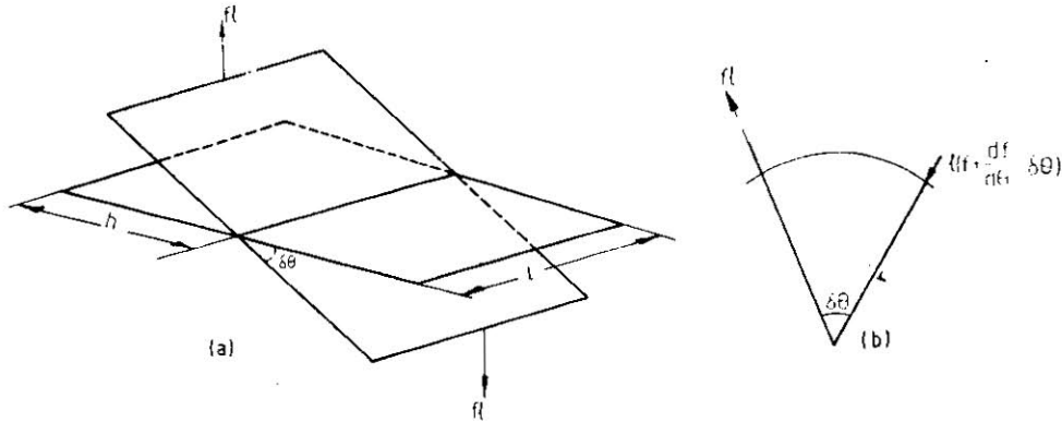
Fig.8 Diagrams used in calculation of the crystallographic orientation effect on \sigma_{sL}
