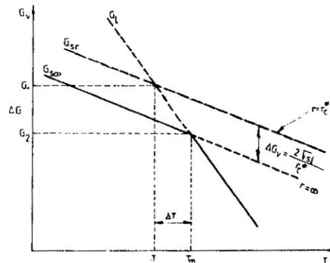
Fig.4 Volume free energy as a function of temperature for solid and liquid phases, showing the origin of the curvature effect
