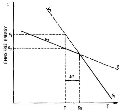
Fig.1.2 Gibbs free energy for solid and liquid phases as a function of temperature near the equilibrium melting point T_m . (the curvature of the G and G_L lines has been neglected)
