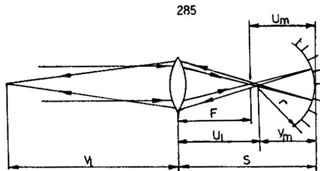
Fig.1- Formation of object at infinity by a lens-curved mirror system.
