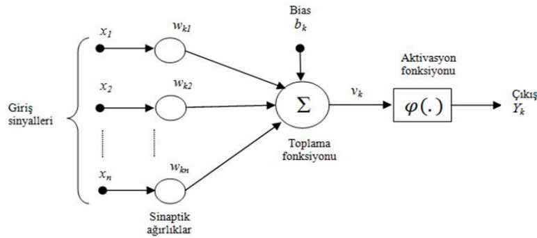
Figure 1: Mathematical Indication of Artificial Neural Network Model
