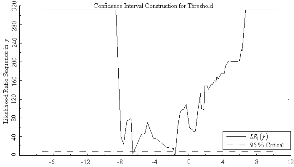
Figure 2: Sample Split: Confidence Interval Construction for Threshold Variable \tilde{\gamma}_{t-1} .
