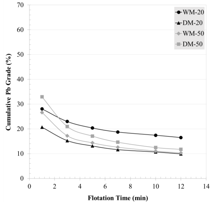
Figure 9. Cumulative Pb Grade over Time
