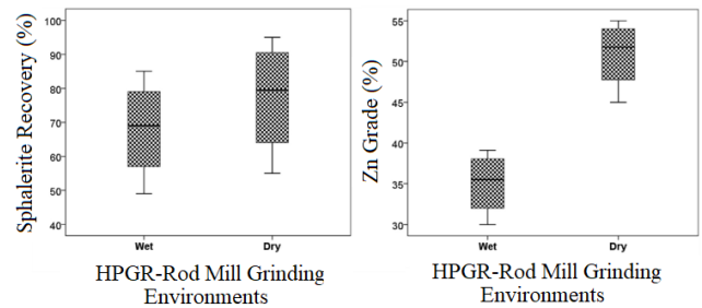
Figure 1. Flotation Performance of Sphalerite in Different Grinding Environments (Chapman et al., 2013)
