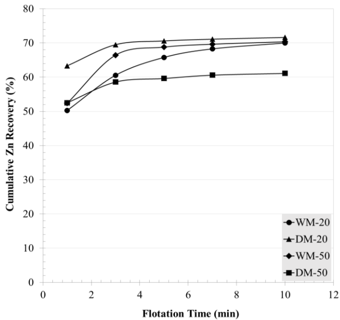
Figure 11. Cumulative Zn Recovery over Time
