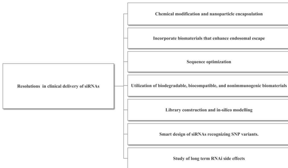
Figure 5. Resolutions in clinical delivery of siRNAs. (adapted from[42])
