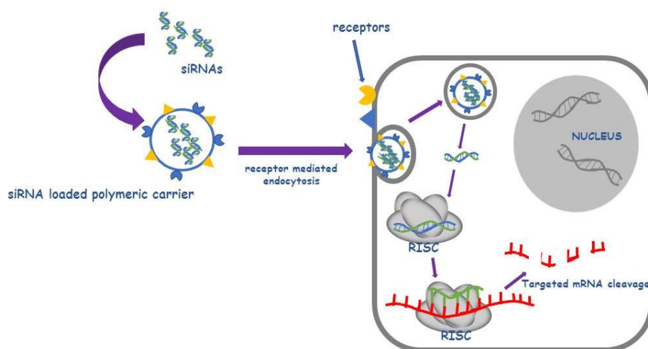
Figure 1. Mechanism of siRNA delivery via polymeric carriers (adapted from [1, 3, 16, 19, 30, 34, 38])
