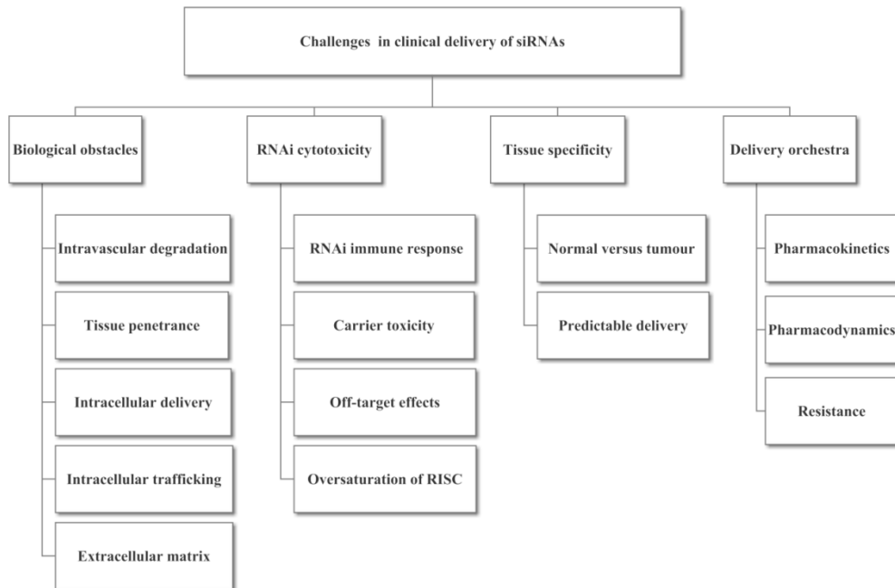
Figure 4. Challenges in clinical delivery of siRNAs.(adapted from [42])
