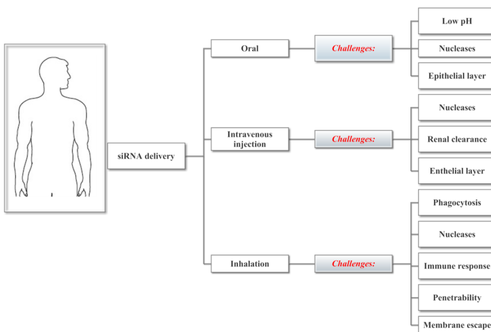
Figure 2. Routes and challenges of siRNA delivery. (adapted from [34, 37, 46, 47])
