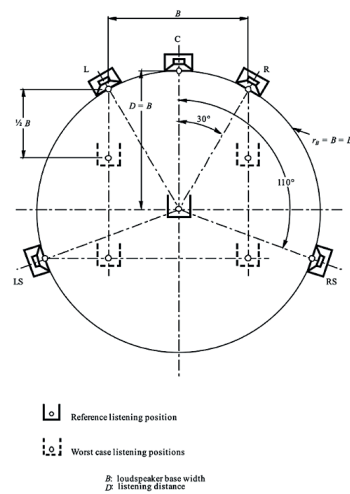
Figure 2. “Test listening arrangement with loudspeakers L/C/R and LS/RS for multichannel sound systems with small impairments” (ITU, 2015, p. 20).
