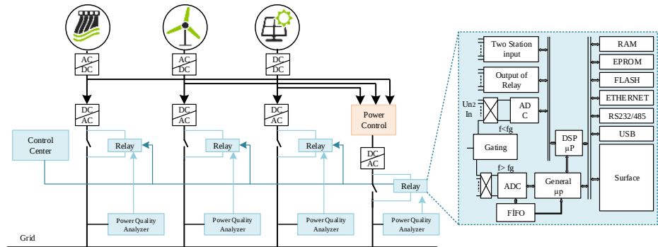
Figure 1. Power mains ports and protection relay analyzer with protection functions
