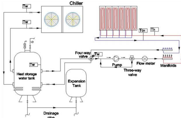
Figure 7. Hydraulic circuit of the test system
