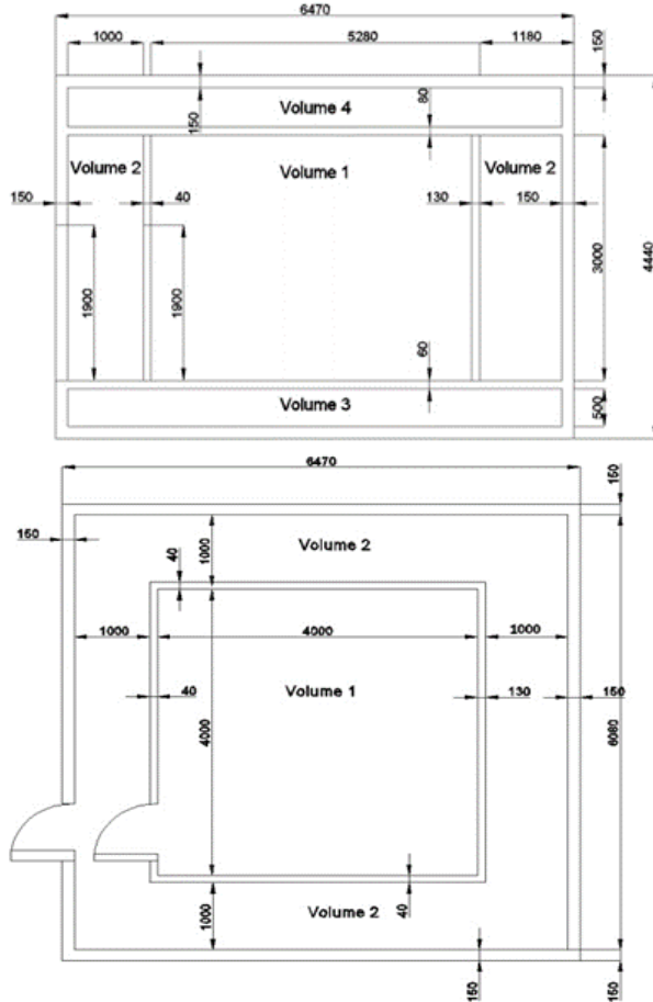
Figure 5. Dimensions of the test chamber (all units are in millimeters)
