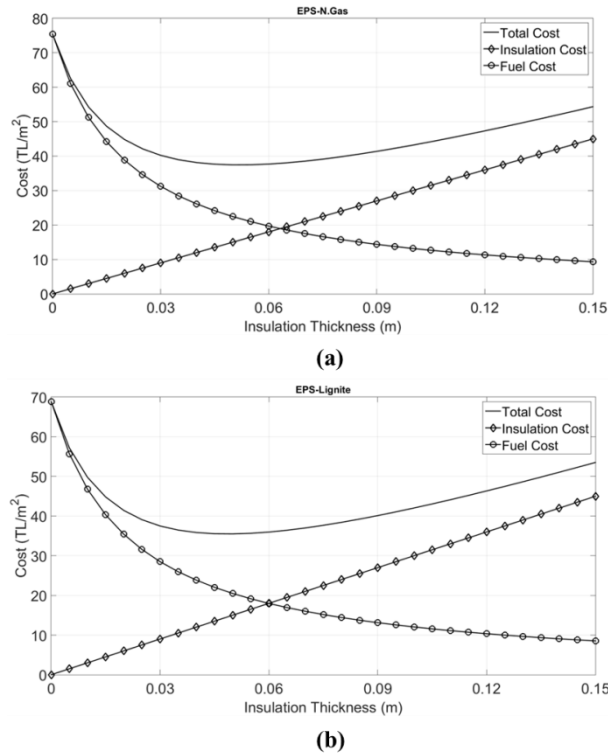
Figure 9. Optimum insulation thickness results of conventional heating systems according to the SDDM a) Natural Gas b) Lignite
