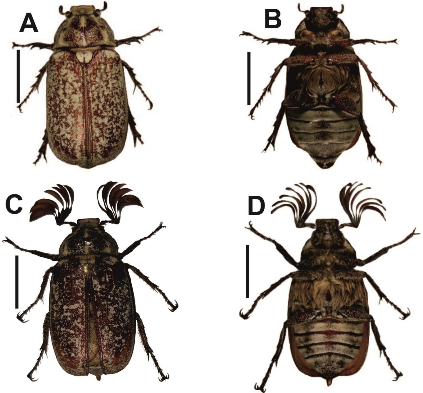
Figure 2. Habitus of P. turkmenoglui Petrovitz, 1965. A) female in dorsal view; B) female in ventral view; C) male in dorsal view; D) male in ventral view. Scale bars: 1 cm (A-D).
