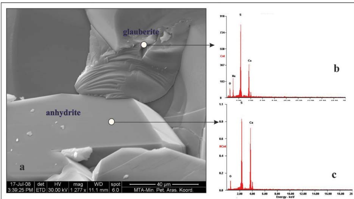
Figure 24- Concoidal fracture surfaces on glauberite mineral grown in anhydrite mineral, (o: measurement point of EDS analysis taken on the crystal) (Balıbaşı-1 drill, 385.30 m XRD figure 18).
