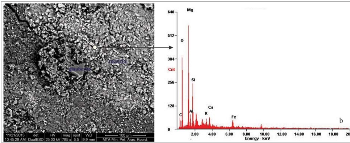
Figure 28- a) General view of the matrix which consists of glauconite layers, b) EDS spectrum of the matrix (o: measurement point of EDS analysis taken on crystal) (Yenidoğan-1 drill, 340 m).
