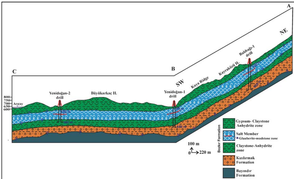
Figure 7- ABC cross section through drillings.
