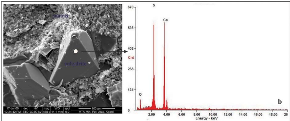
Figure 22- a) Euhedral anhydrite crystal within matrix, b) EDS spectrum of the anhydrite mineral, (o: measurement point of EDS analysis taken on the crystal), (Yenidoğan-2 drill, 366.1 m, XRD figure 19).
