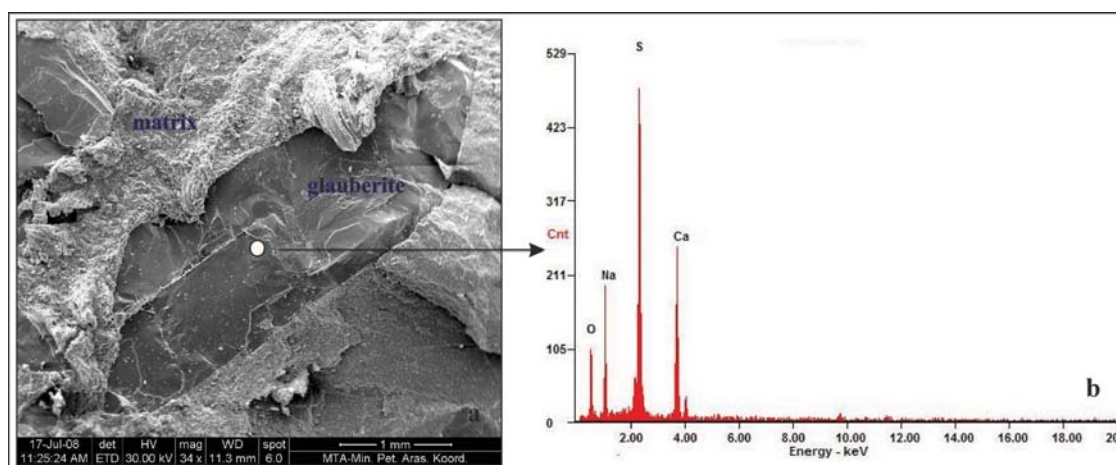
Figure 20- a) Euhedral glauberite crystal within matrix, b) EDS spectrum of the glauberite mineral (o: measurement point of EDS analysis taken on the crystal) (Balıbağı-1 drill, 385.30 m, XRD figure 18).
