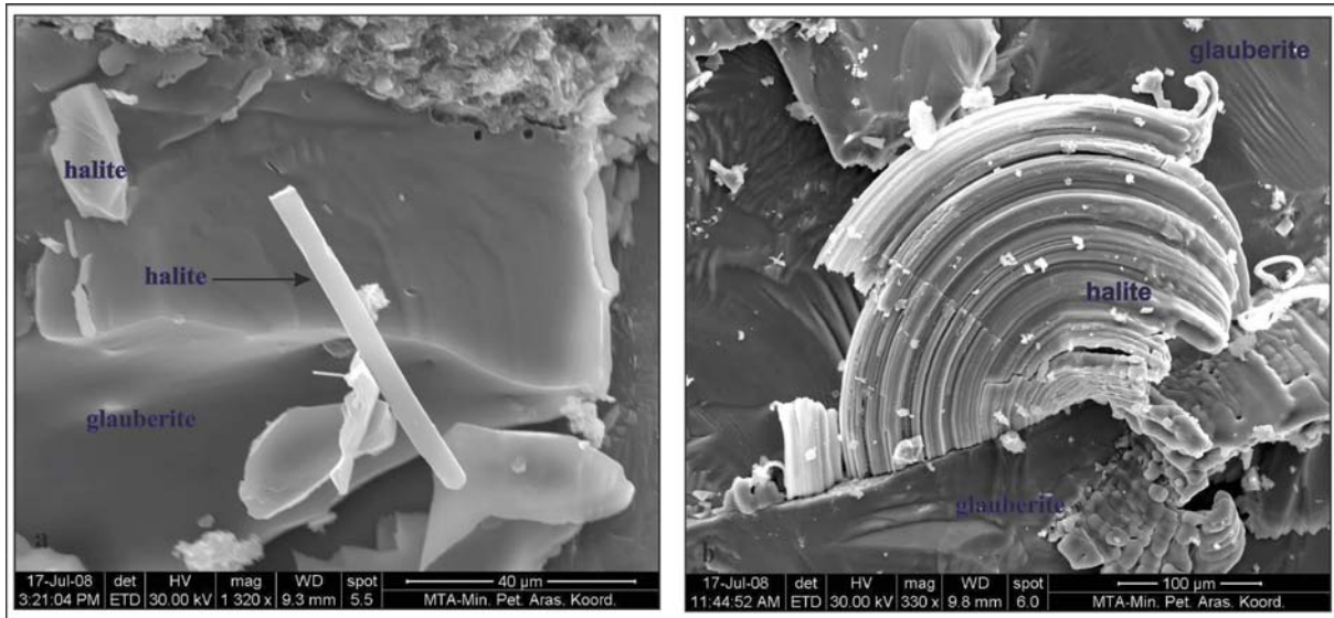
Figure 26- Crystallized halite forms on glauberite mineral, a) rod like halite crystal, b) concentric halite crystal (a, b: Balıbağı-1 drill, 385.30 m, XRD figure 18).
