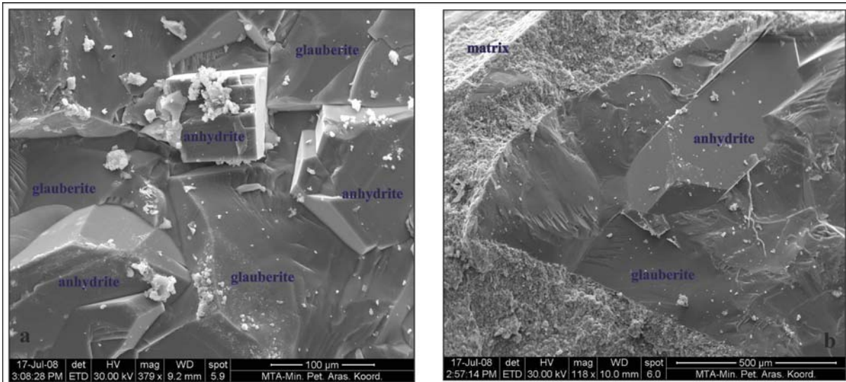
Figure 23- a) SE views of glauberite-anhydrite crystals, b) SE view of euhedral anhydrite mineral within glauberite mineral. (Balıbaşı-1, 385.30 m, XRD figure 18).
