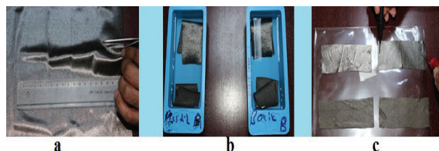
Figure 8. Preparing and measuring of the patterns (a: cutting of the patterns, b: putting the samples into solution, c: measuring the resistance of patterns)
