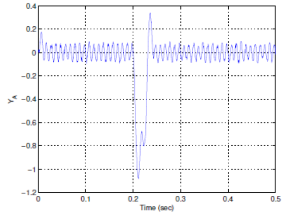
Figure 4b. Rotor position (Volts) for decentralized PID Control
