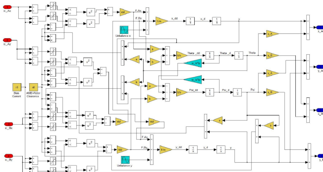
Figure 3. Nonlinear rotor/electromagnetic bearing model in Simulink
