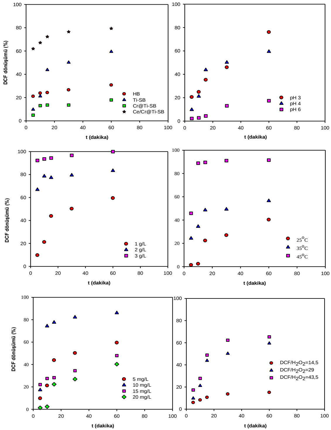
Şekil 6. Sütunlu bentonit katalizörlerin katalitik performansları (a) pH 4, t=25^{\circ}\text{C} , m_{\text{kat}}=1 \text{ g/L} , \text{H}_2\text{O}_2/\text{DCF}=29 ve 5 \text{ mg/L} DCF (b) pH 3, 4 ve 6, t=25^{\circ}\text{C} , m_{\text{kat}}=1 \text{ g/L} , \text{H}_2\text{O}_2/\text{DCF}=29 ve 5 \text{ mg/L} DCF (c) m_{\text{kat}}=1 \text{ g/L} , 2 \text{ g/L} ve 3 \text{ g/L} , pH 4, T=25^{\circ}\text{C} , \text{H}_2\text{O}_2/\text{DCF}=29 ve 5 \text{ mg/L} DCF (d) T=25^{\circ}\text{C} , 35^{\circ}\text{C} ve 45^{\circ}\text{C} , pH 4, m_{\text{kat}}=1 \text{ g/L} , \text{H}_2\text{O}_2/\text{DCF}=29 ve 5 \text{ mg/L} DCF (e) pH 4, T=25^{\circ}\text{C} , m_{\text{kat}}=1 \text{ g/L} , \text{H}_2\text{O}_2/\text{DCF}=29 ve 5-20 \text{ mg/L} DCF (f) \text{H}_2\text{O}_2/\text{DCF}=14,5 ; 29 ve 43,5 , pH 4, T=25^{\circ}\text{C} , m_{\text{kat}}=1 \text{ g/L} , 5 \text{ mg/L} DCF
