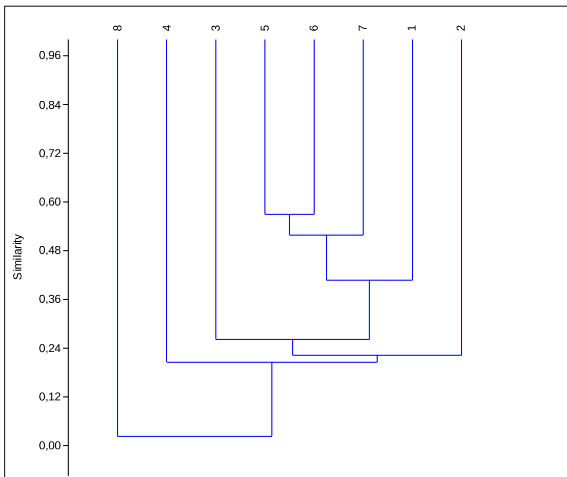
Figure 2. Similarity diagram of Arrenurus species in some countries in the Palearctic Region (1. Turkey, 2. Iran, 3. Greece, 4. Bulgaria, 5. France, 6. Netherlands, 7. Belgium, 8. Japan)
