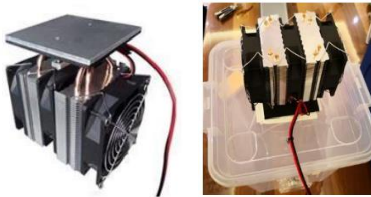
Figure 7. Thermoelectric cooler module block and water tank with copper, aluminum cooler, and fan circulation used in the system (Özcan, Çelebi & Arpacioğlu, 2022)
