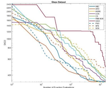
(c) Glass Veri Seti (Glass Dataset)
