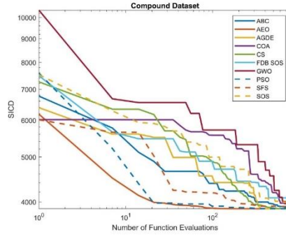
(b) Compound Veri Seti (Compound Dataset)
