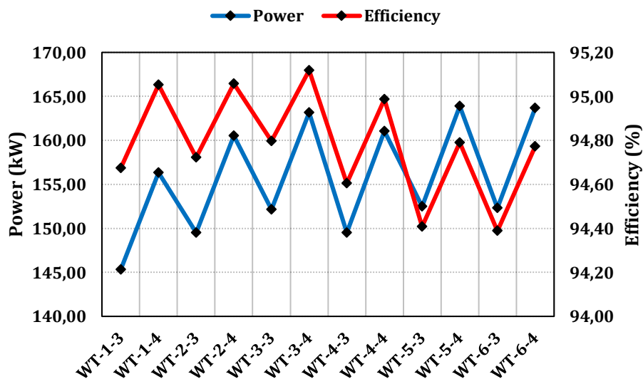
Figure 4. Shaft power and efficiency of SynRM winding models with 3 and 4 flux barriers.
