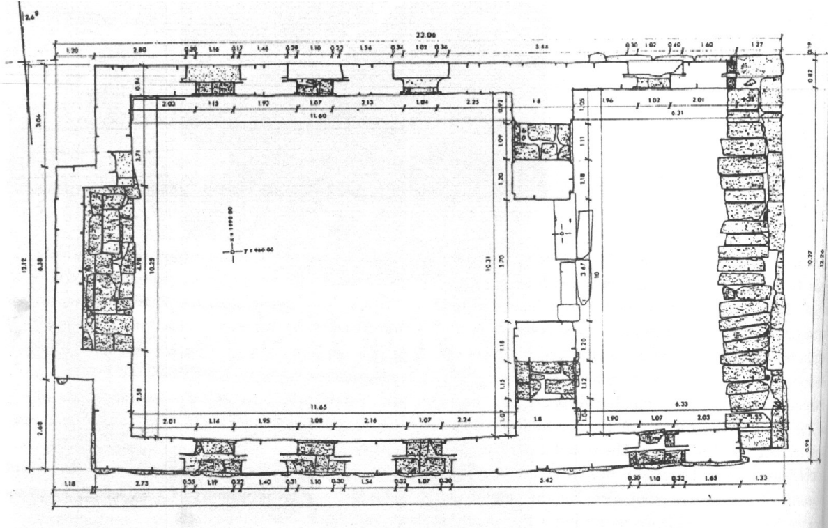
Şekil 6. Labraunda Andron A plan (Hellström, 1994: fig. 14).
