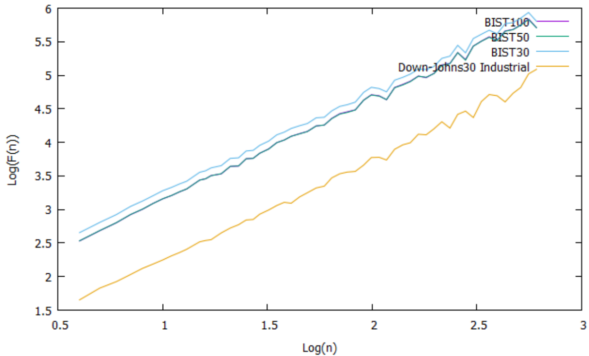
Figure 2 : Detrended Fluctuation Analysis
