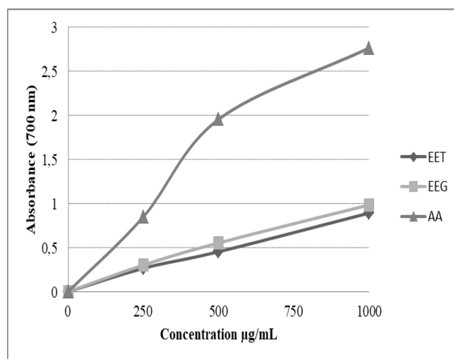
Figure 3. Total reductive potential of different concentrations (250–1000 \mu\text{g/mL} ) of EEG ( r^2 : 0.9973), EET ( r^2 : 0.9935), and reference antioxidant: ascorbic acid using spectrophotometric detection of the \text{Fe}^{3+} – \text{Fe}^{2+} transformations. In the presence of reductants, \text{Fe}^{3+} /ferricyanide complex reduces to the ferrous form (EET: ethanolic extract turmeric, EEG: ethanolic extract ginger, AA; ascorbic acid, Absorbance was the mean \pm SD ( n=3 ) p < 0.01 ).
