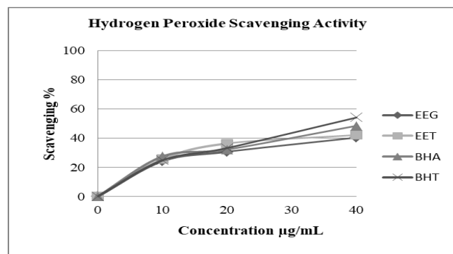
Figure 2. Scavenging effect of EET, EEG, BHA and BHT on H_2O_2 , at different concentrations (10–40 \mu\text{g/mL} ) (EET: ethanolic extract turmeric, EEG: ethanolic extract ginger, BHA: butylated hydroxyanisole, BHT: butylated hydroxytoluene, H_2O_2 : Hydrogen Peroxide, The Scavenging (%) was the mean \pm SD ( n=3 ) p < 0.05 ).
