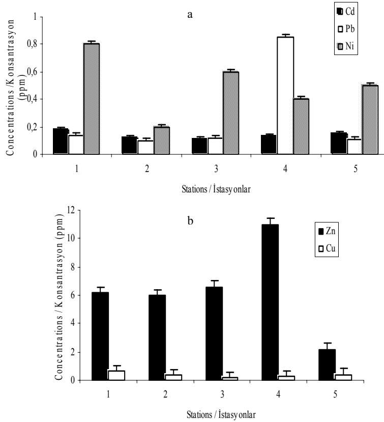
Figure 1: Mean a) cadmium, nickel and lead, b) zinc and copper concentrations in honey bee samples and standard error bars
