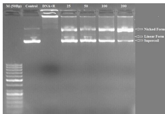
FIGURE 2. DNA protecting activity of TME. M: Marker, Negative control (DNA + R): pBR322 + OH radical, 25, 50, 100 and 200 µg / mL doses + OH radical.
