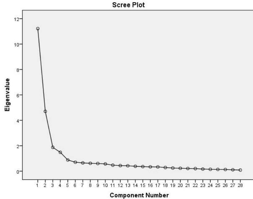
Figure 2. Scree Plot
