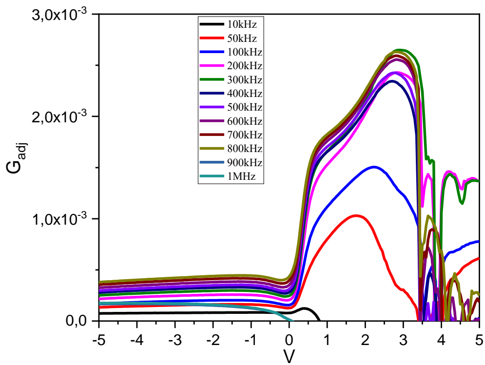
Figure 7: G_{adj} - V characteristics of 6% Mn doped cadmium oxide photodiodes.
