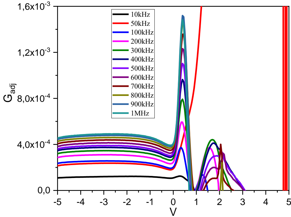
Figure 8: G_{adj} - V characteristics of 10% Mn doped cadmium oxide photodiodes.
