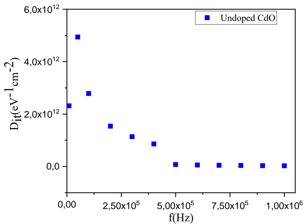
Figure 9: Density of interface states of undoped cadmium oxide photodiodes.
