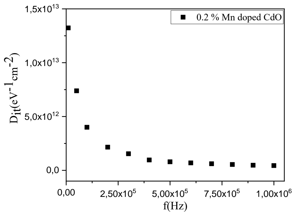
Figure 10: Density of interface states of 0.2% Mn doped cadmium oxide photodiodes.
