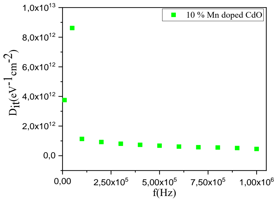
Figure 12: Density of interface states of 10% Mn doped cadmium oxide photodiodes.
