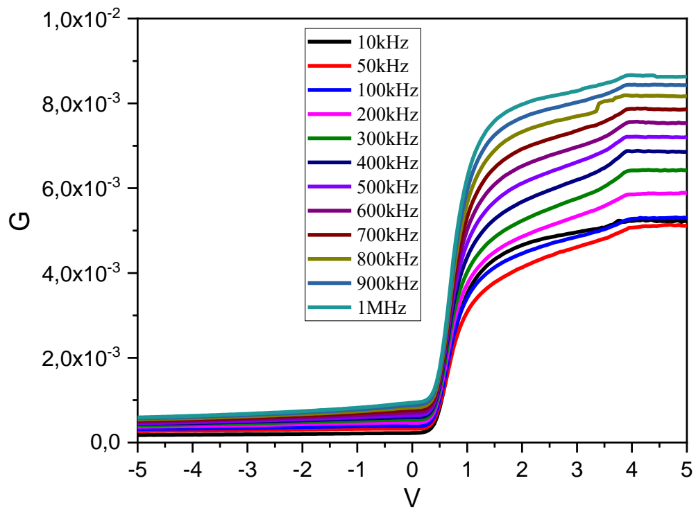
Figure 2: G - V characteristics of 0.2% Mn doped cadmium oxide photodiodes.
