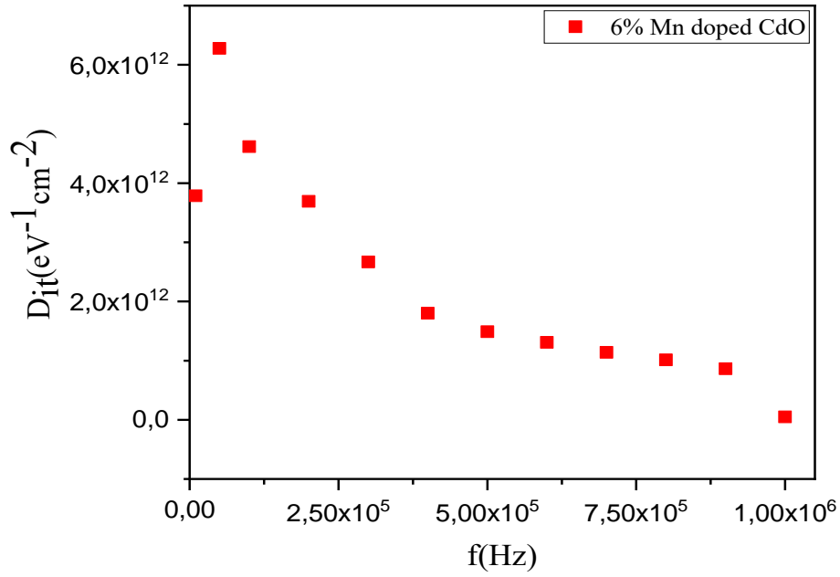
Figure 11: Density of interface states of 6% Mn cadmium oxide photodiodes
