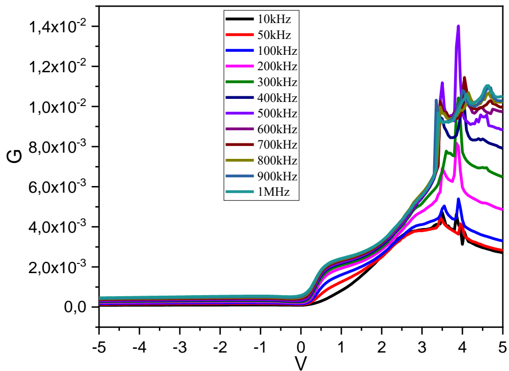
Figure 3: G - V characteristics of 6% Mn doped cadmium oxide photodiodes.
