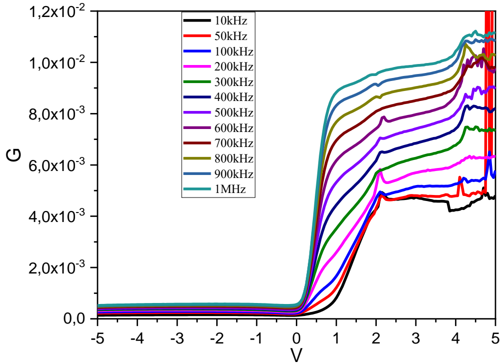
Figure 4: G - V characteristics of 10% Mn doped cadmium oxide photodiodes.
