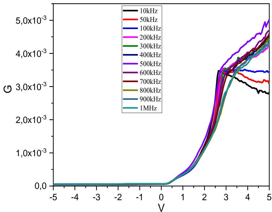
Figure 1: G - V characteristics of
