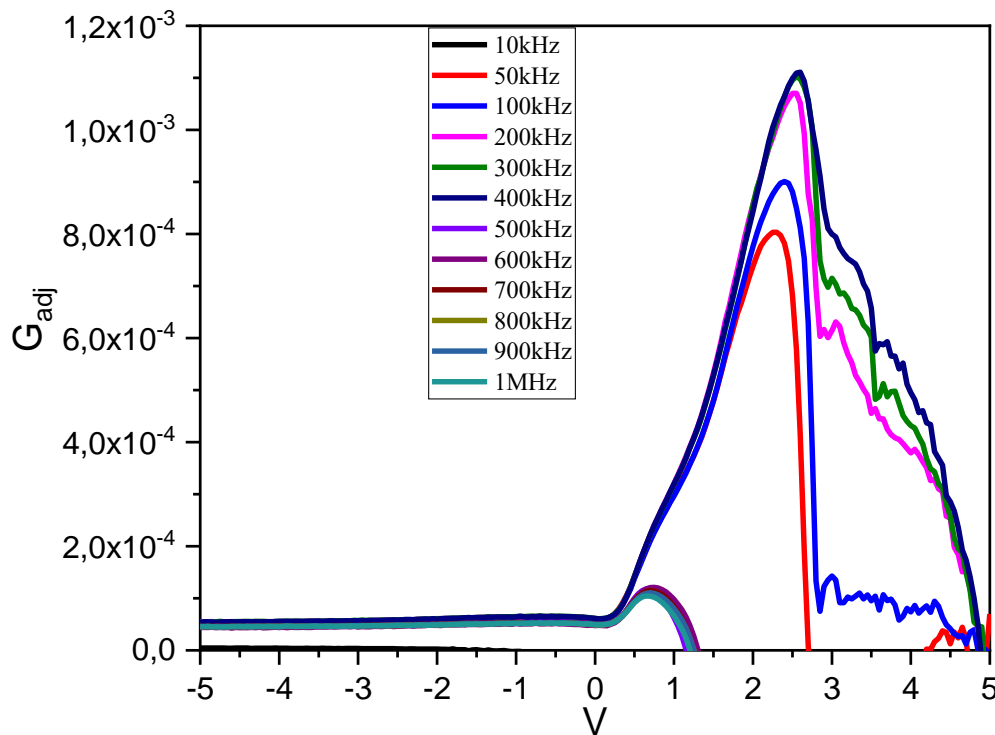
Figure 5: G_{adj} - V characteristics of undoped cadmium oxide photodiodes.
