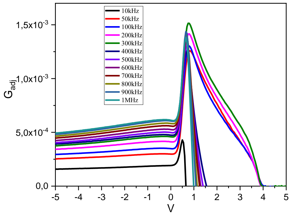
Figure 6: G_{adj} - V characteristics of 0.2% Mn doped cadmium oxide photodiodes.
