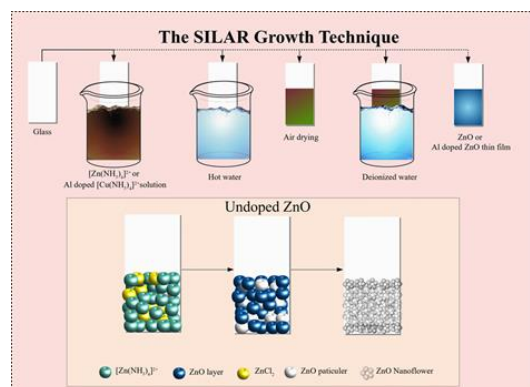
Figure 1. Mechanism of growth of ZnO thin films on ITO substrate by SILAR technique
